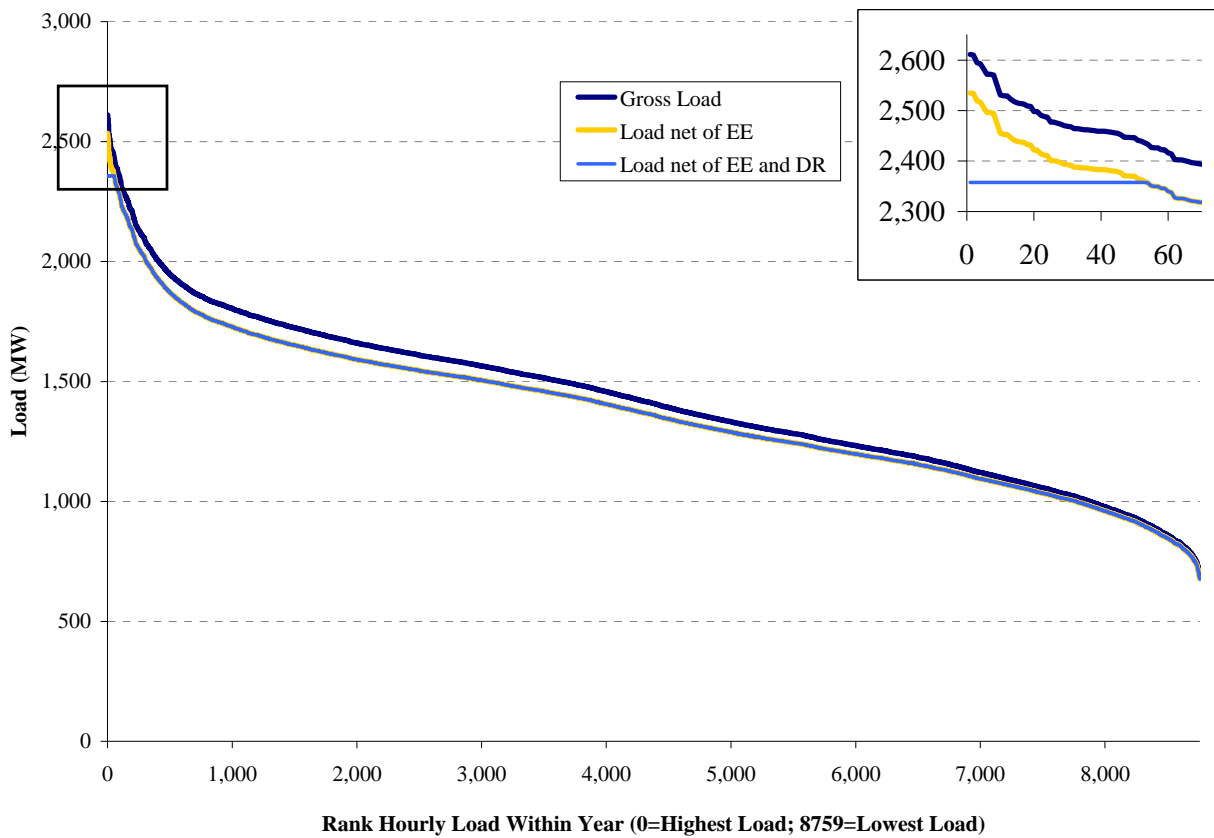
Figure G.22: Net Load with Reference DSM in the Current Trends Scenario: 2011 SW-CT Example
