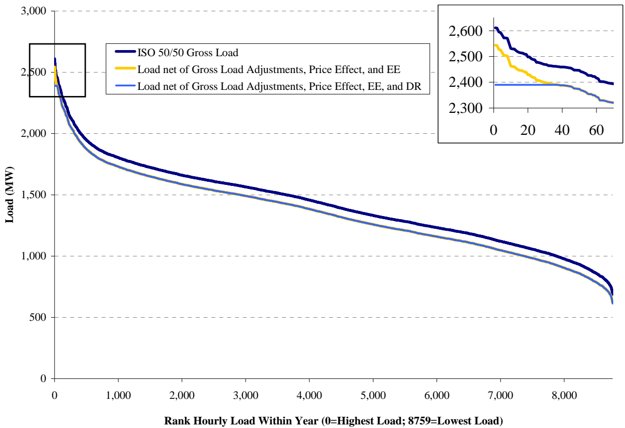
Figure G.26: Net Load with Gross Load Adjustments, Fuel Price Effect, and Reference DSM in High Fuel/Growth Scenario: 2011 SW-CT Example
